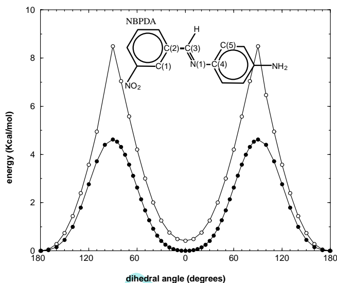
FIG. 5 The molecular structure of NBPDA (inset) and potential energy curves for internal rotations of NBPDA. Solid circles: rotation about the (C_3, N_{(1)}, C_4, C_5) dihedral angle. Open circles: rotation about the (C_1, C_2, C_3, C_5) dihedral angle.
